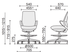
High Chair with High Back
