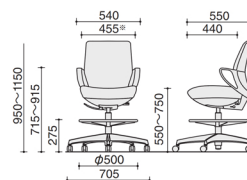
High Chair with Low Back
